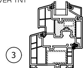
HORIZ. SECTION FIXED OVER TNT
