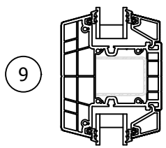
HORIZ. SECTION FIXED OVER FIXED
