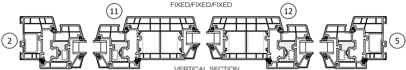
VERTICAL SECTION TNT/FIXED/TNT
