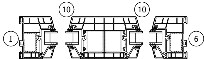
VERTICAL SECTION FIXED/FIXED/FIXED
