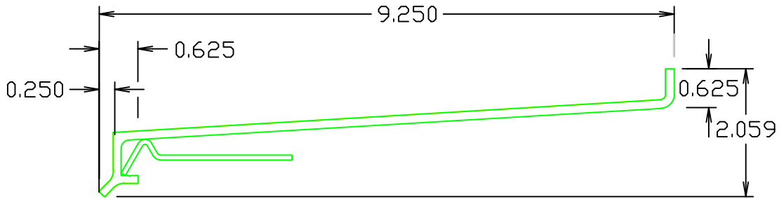
9 1/4" ALOCA SILL & CLIP
