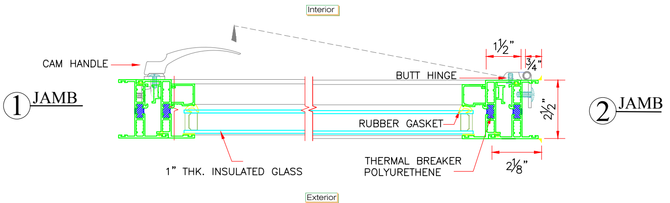
TYPICAL SECTIONAL DETAILS
