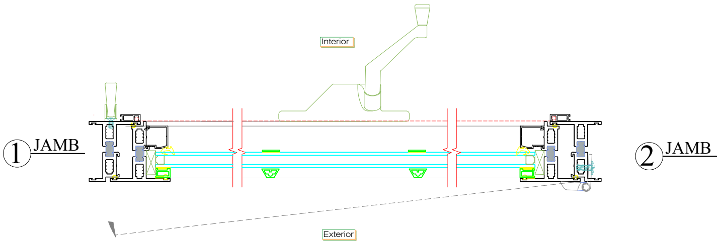
TYPICAL SECTIONAL DETAILS
