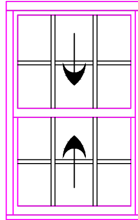
ADHESIVE FLAT SDL INTERIOR WITH EXTERIOR APPLIED GRID FRAME CALL FOR OPTIONAL SDL PROFILES
