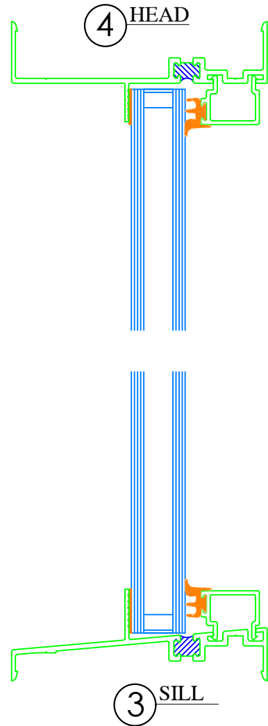
Typical Vert. Sectional Details
