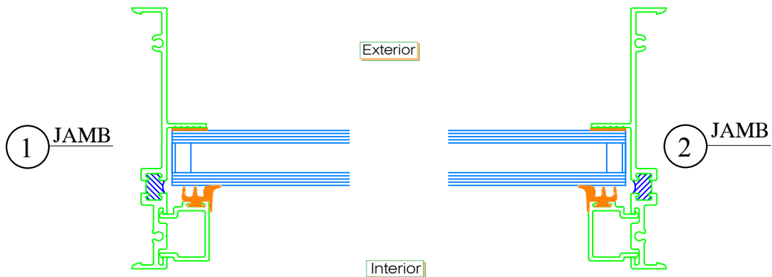
Typical Horiz. Sectional Details
