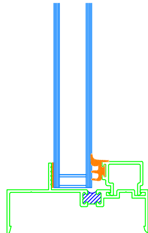
Typical Vert. Sectional Details
