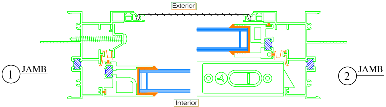
Typical Horiz. Sectional Details
