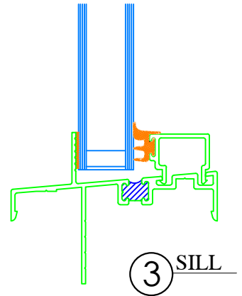
Typical Vert. Sectional Details
