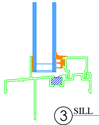
Typical Vert. Sectional Details
