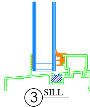
Typical Vert. Sectional Details
