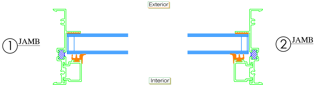
Typical Horiz. Sectional Details
