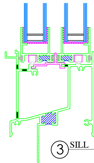
Typical Vert. Sectional Details
