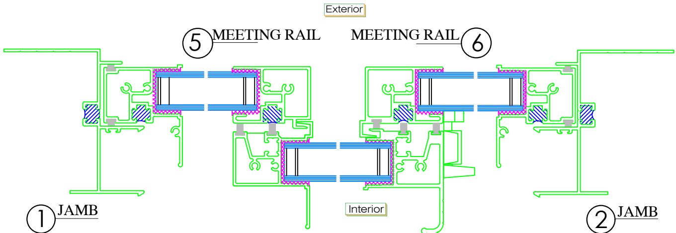
Typical Horiz. Sectional Details
