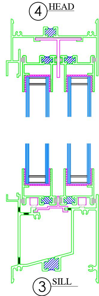
Typical Vert. Sectional Details
