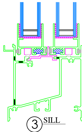
Typical Vert. Sectional Details
