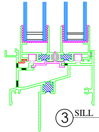
Typical Vert. Sectional Details
