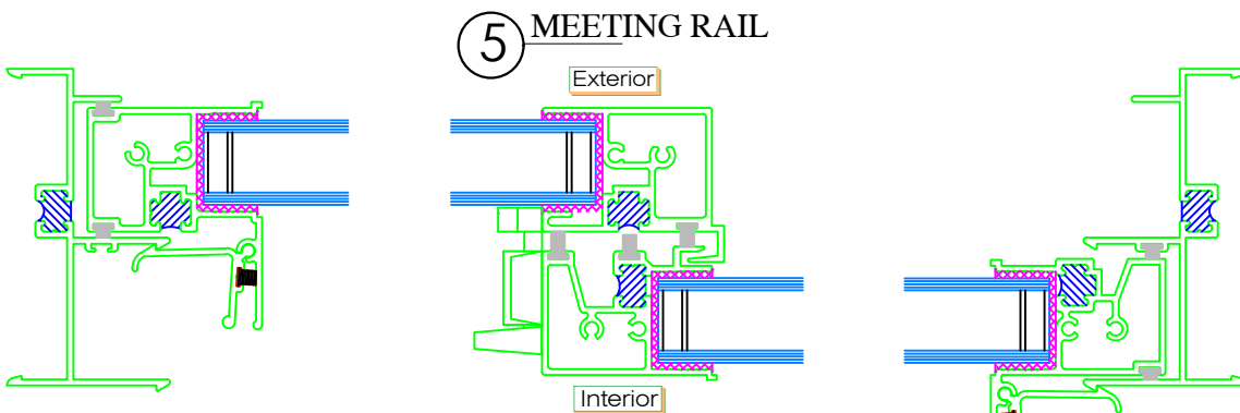
Typical Horiz. Sectional Details
