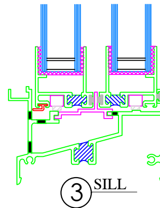
Typical Vert. Sectional Details
