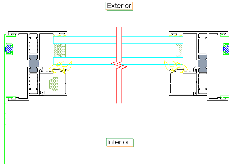
TYPICAL SECTIONAL DETAILS
