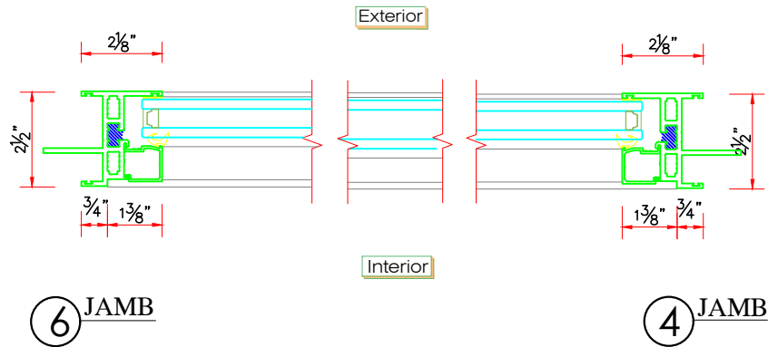
TYPICAL HORIZ. SECTIONAL DETAILS SCALE : 3" = 1'-0"
