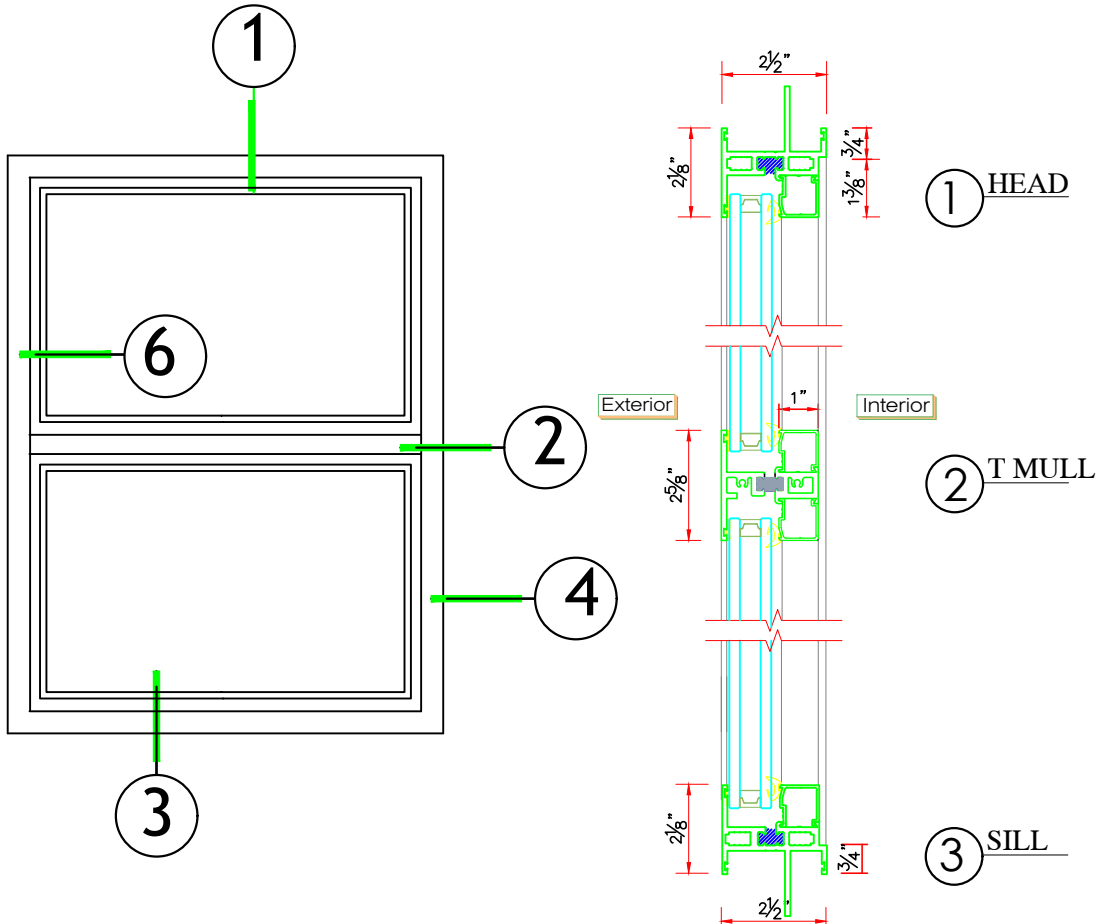
TYPICAL VERT. SECTIONAL DETAILS SCALE : 3" = 1'-0"
