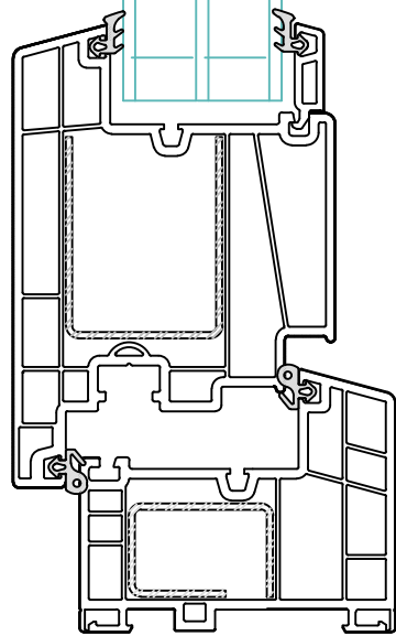
3 SILL SECTION
