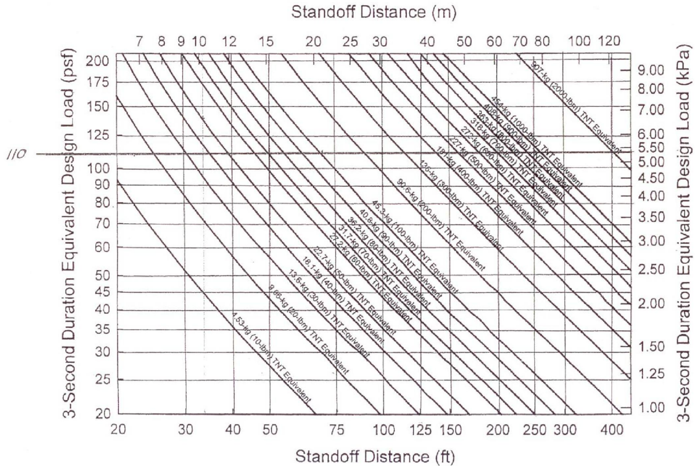
FIG. 1 Graphical Relationship Between Standoff Distance, TNT Charge Mass, and 3-Second Equivalent Design Load
